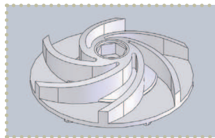
Impeller Design
