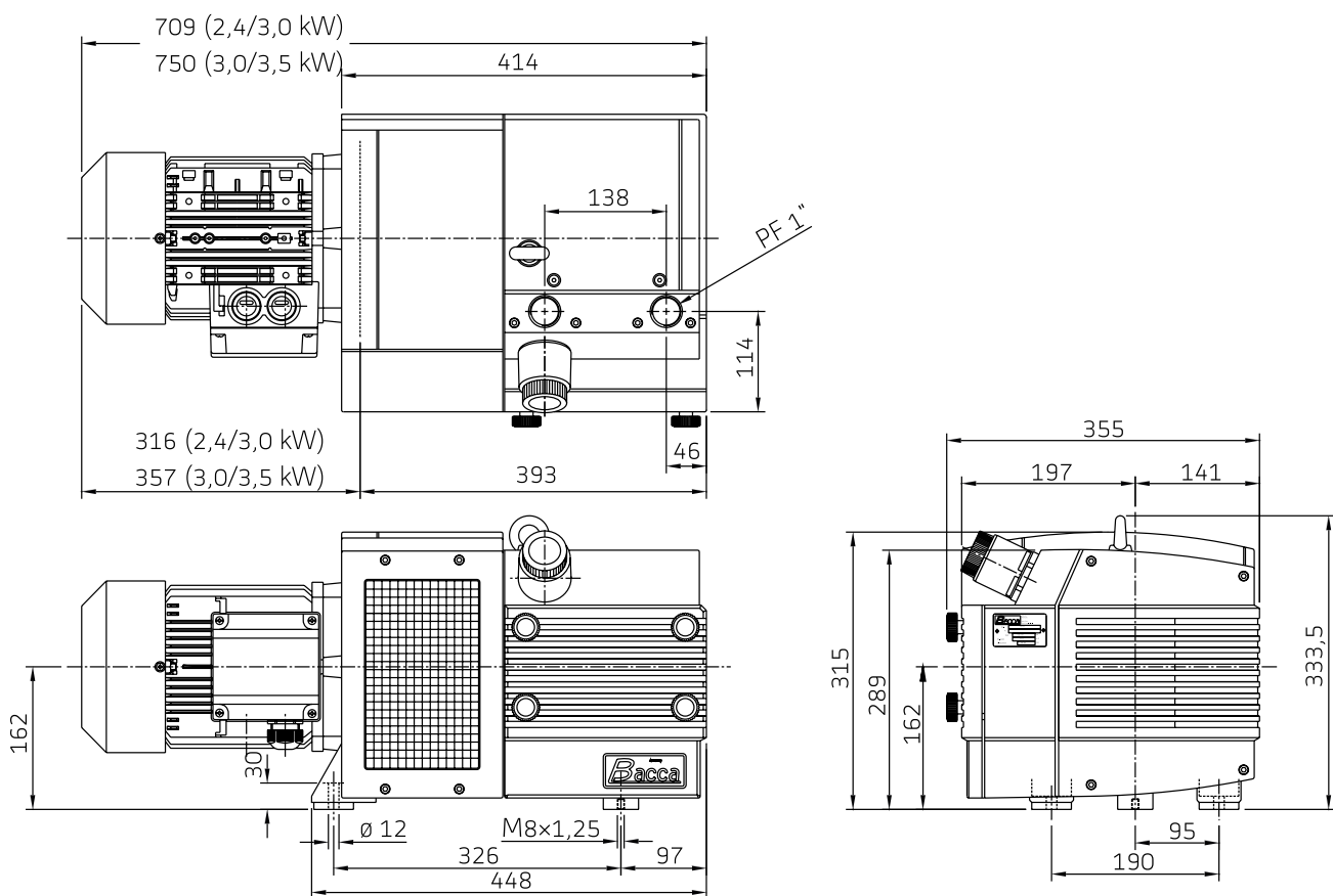
Vane rotary compressor DRT 3140
